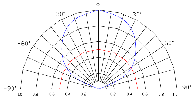
Relative Lumionous Intensity(LOP @max=1)
