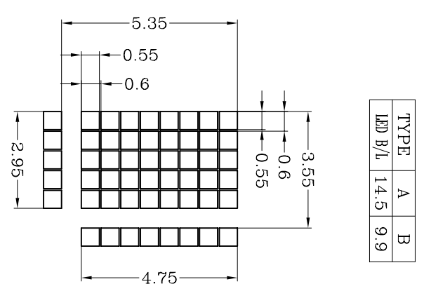
DOTS DETAIL SCALE 6:1
